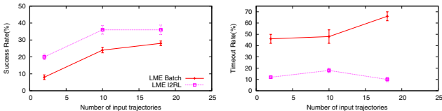
Figure 6: Success and timeout rates for experiments involving physical robots at less than 30% observability.
